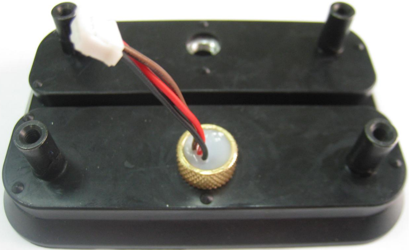
Sensor installed in a 4x2 vacuum cup (ORRVACUP-4x2-001)
